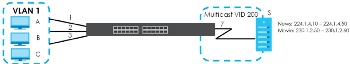
Figure 172 MVR Configuration Example
